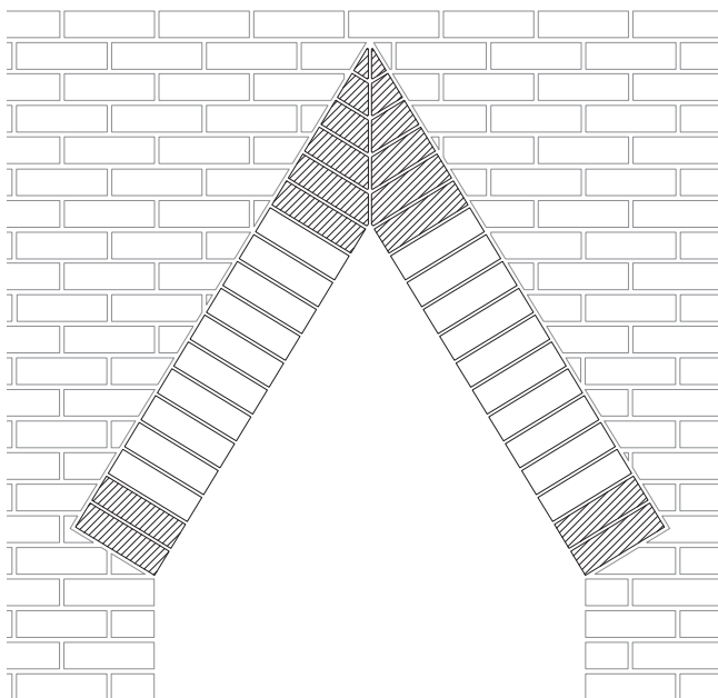
A triangular pseudo-arch of two courses of stretchers at an acute angle, lean together at a mitred apex, common in Anglo-Saxon architecture, also called pediment or mitre arch.
